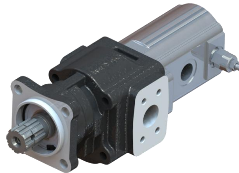
GP40/SP20 tandem pump
