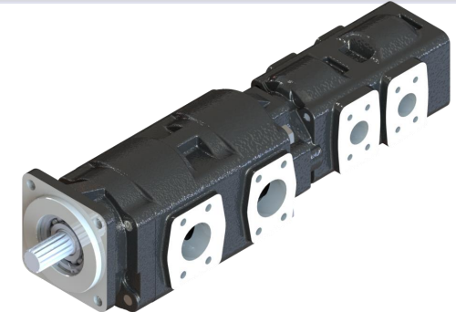
GP60/GP60 / GP60/GP60 quadruple pump
