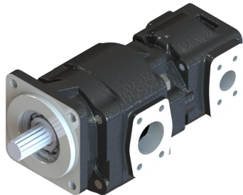
GP60/GP40 tandem pump
